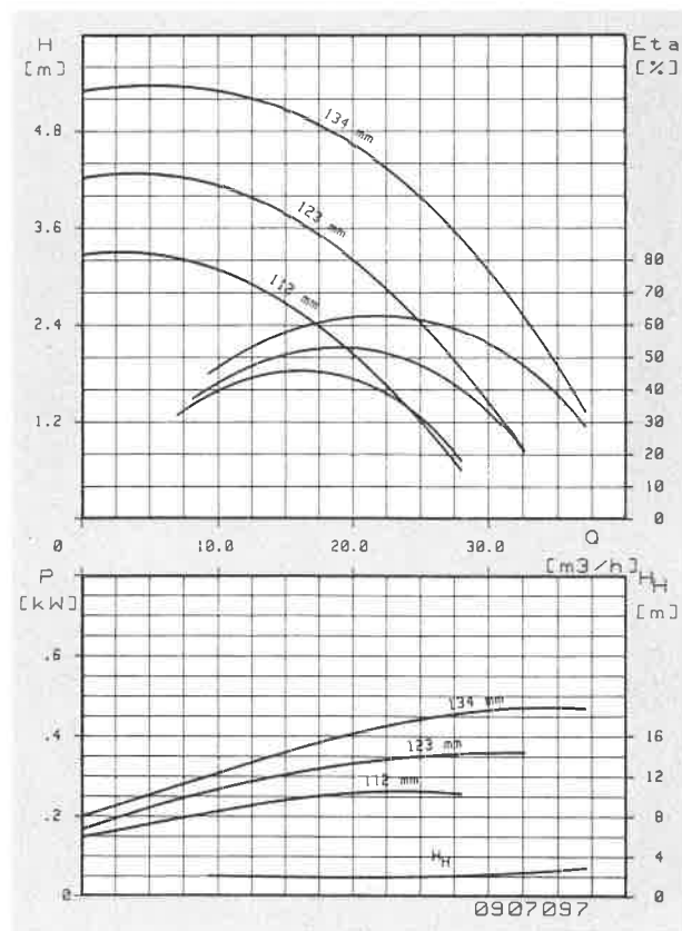
CM 50-125 n = 1450 \text{ min}^{-1} DN 65/50
