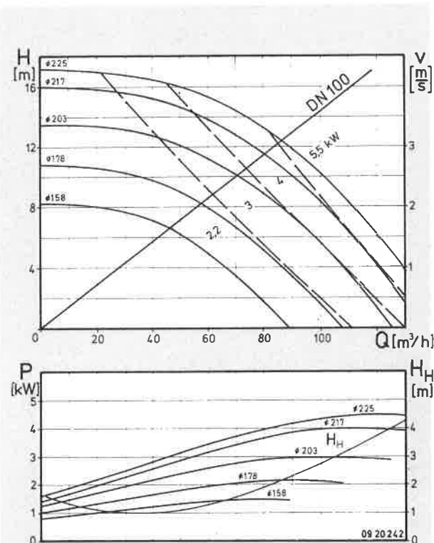
CLM 100 n = 1450 \text{ min}^{-1} DN 100
