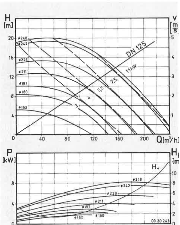
CLM 125 n = 1450 \text{ min}^{-1} DN 125
