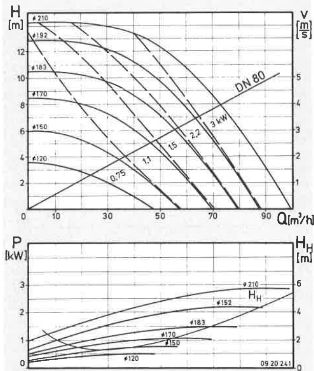
CLM 80 n = 1450 \text{ min}^{-1} DN 80
