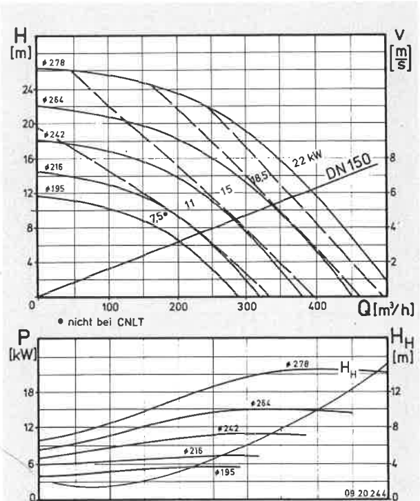
CLM 150 n = 1450 \text{ min}^{-1} DN 150
